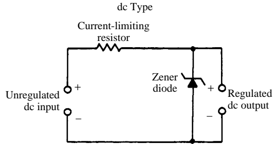
zener-diode voltage reference
