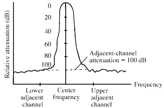
adjacent-channel attenuation
