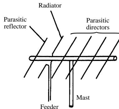
yagi antenna
