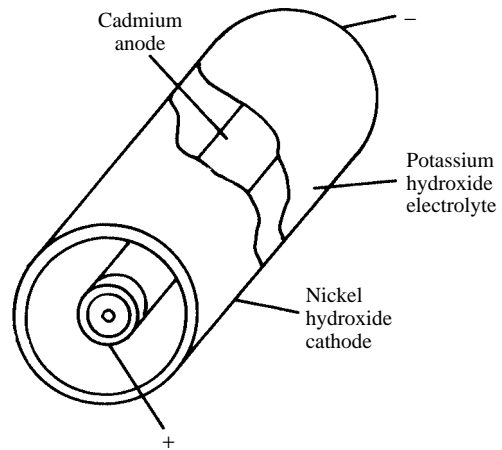
nickel-cadmium cell
