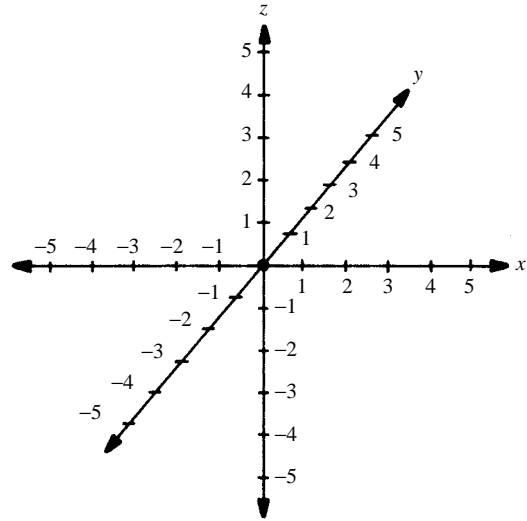
Cartesian three-space
