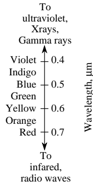
color spectrum
