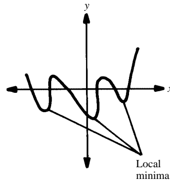
minima
