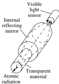
Cerenkov radiation
