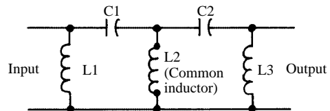
common-inductor coupling
