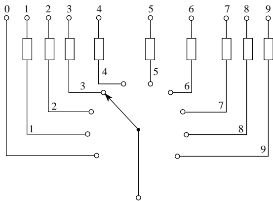
decade box
