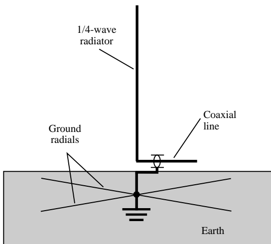
quarter-wave antenna
