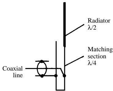
J antenna
