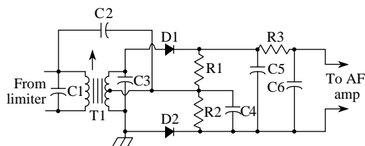
discriminator
