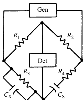
Wien bridge
