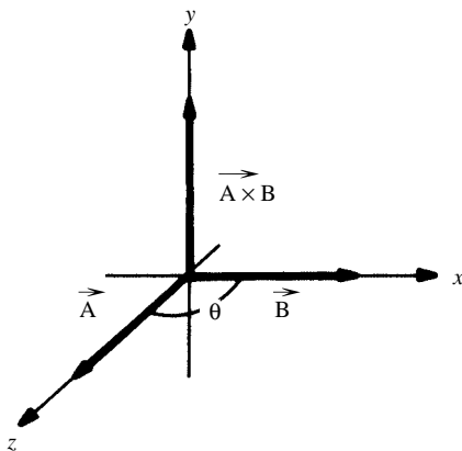
cross product
