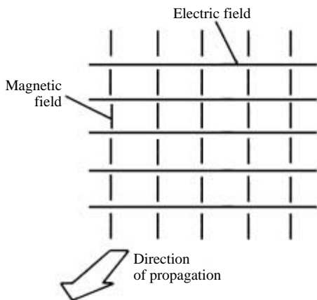
electromagnetic field
