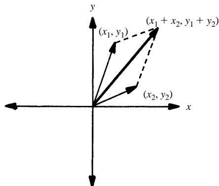
vector addition
