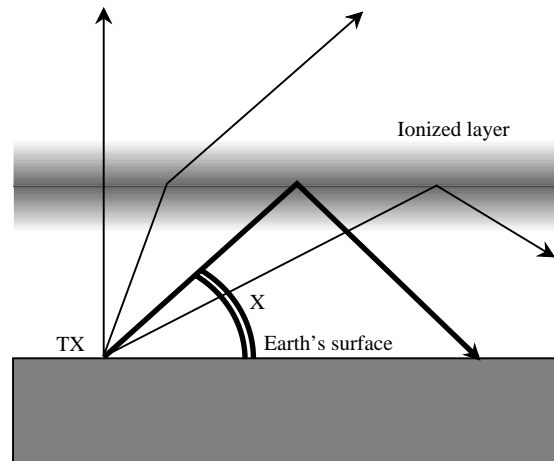
critical angle, 1
