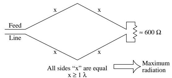
diamond antenna
