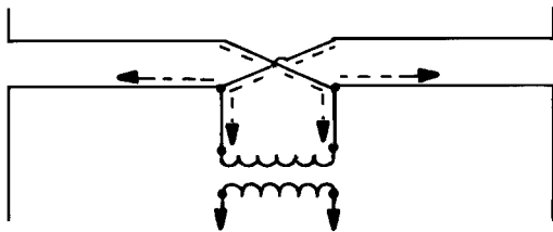
Adcock antenna
