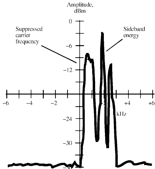
upper sideband
