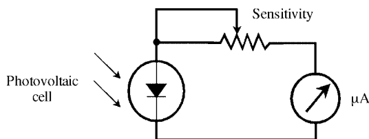
illuminometer
