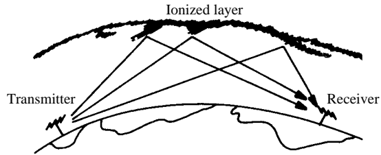
multipath reception
