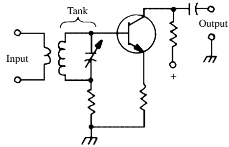
input tank
