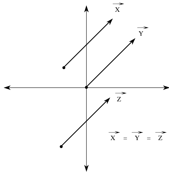
equal vectors
