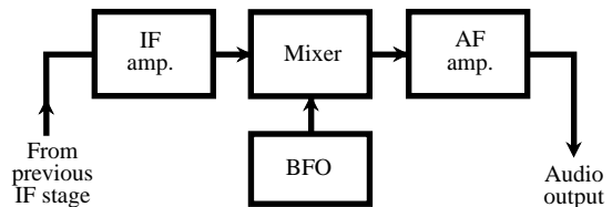
beat-frequency oscillator
