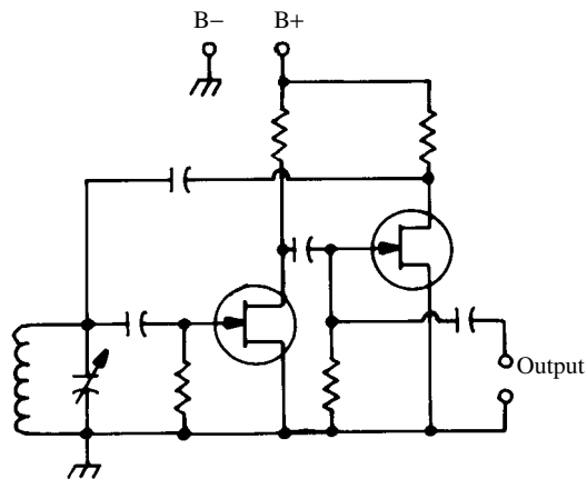
Franklin oscillator
