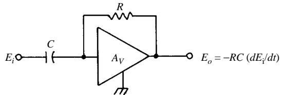
differentiator, 2
