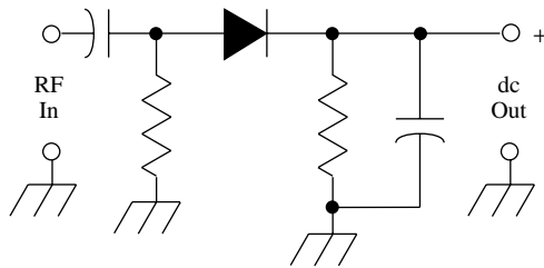
signal rectification
