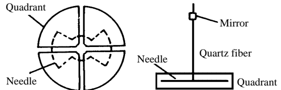
quadrant electrometer
