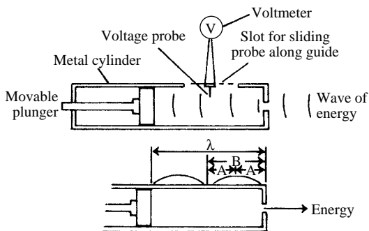
waveguide wavemeter
