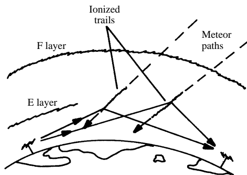
meteor-trail reflections
