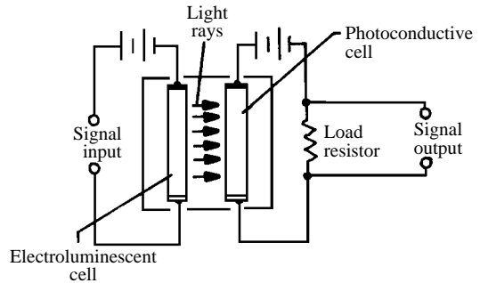
lumistor
