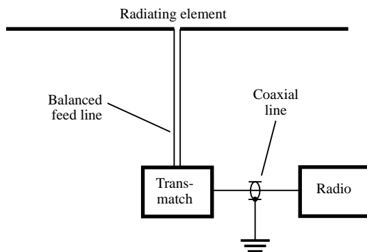
multiband antenna
