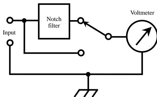
distortion meter
