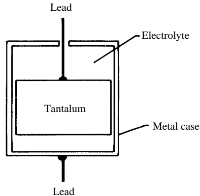
tantalum capacitor
