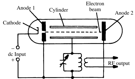
Heil oscillator
