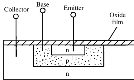
planar transistor
