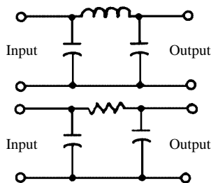
pi filters
