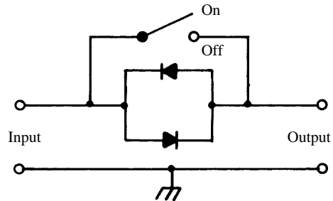
threshold detector
