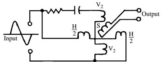
Helmholtz coil
