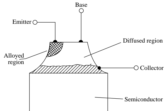
mesa transistor
