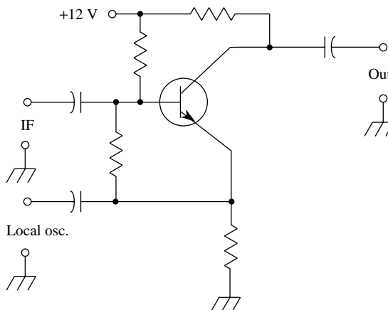
product detector
