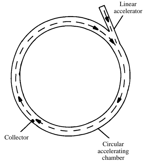
synchrotron
