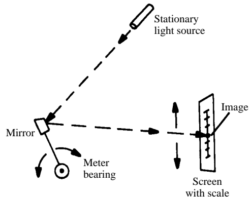
optical lever
