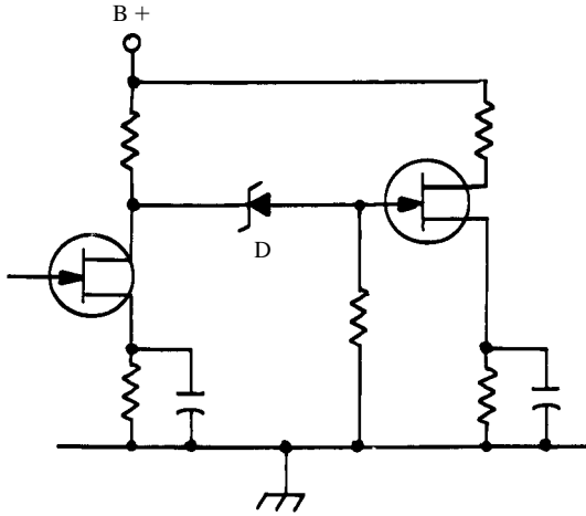
zener-diode coupling element
